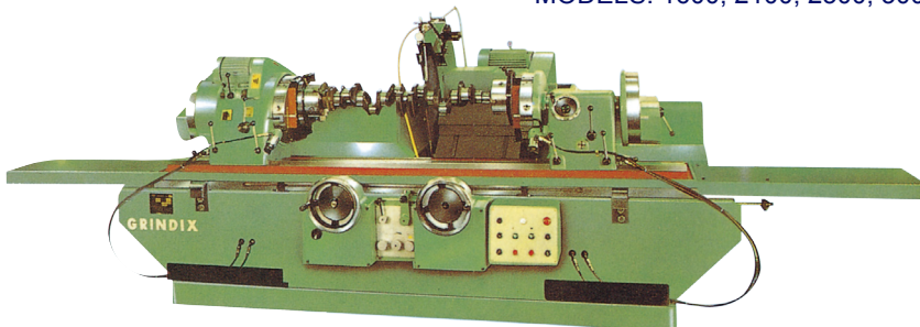
Hydraulic Crankshaft Grinder MODELS: 1600, 2100, 2500, 3000
