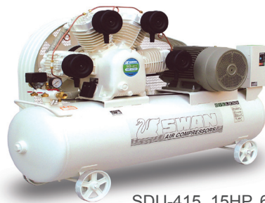
SDU-415, 15HP, 67 CFM
